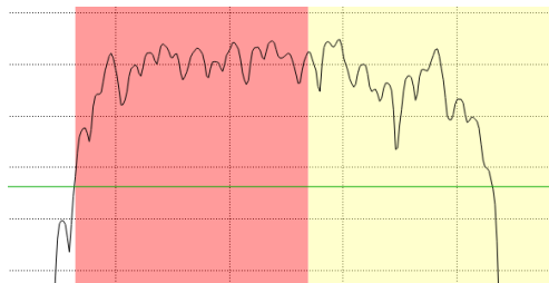
Figure 40: A signal breaking a flat baseline threshold and falling partially within an exclusion zone (the yellow shaded portion). Only the unexcluded part of the signal is considered an event (the red shaded portion).
