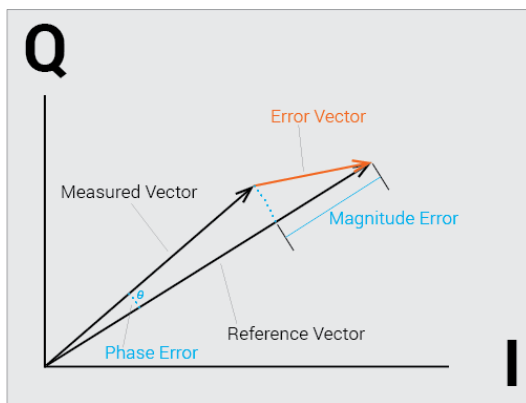
Figure 21: Visualization of the EVM, Magnitude and Phase Error Calculations
