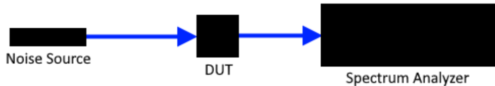
Figure 53: Noise figure DUT measurement step setup.
