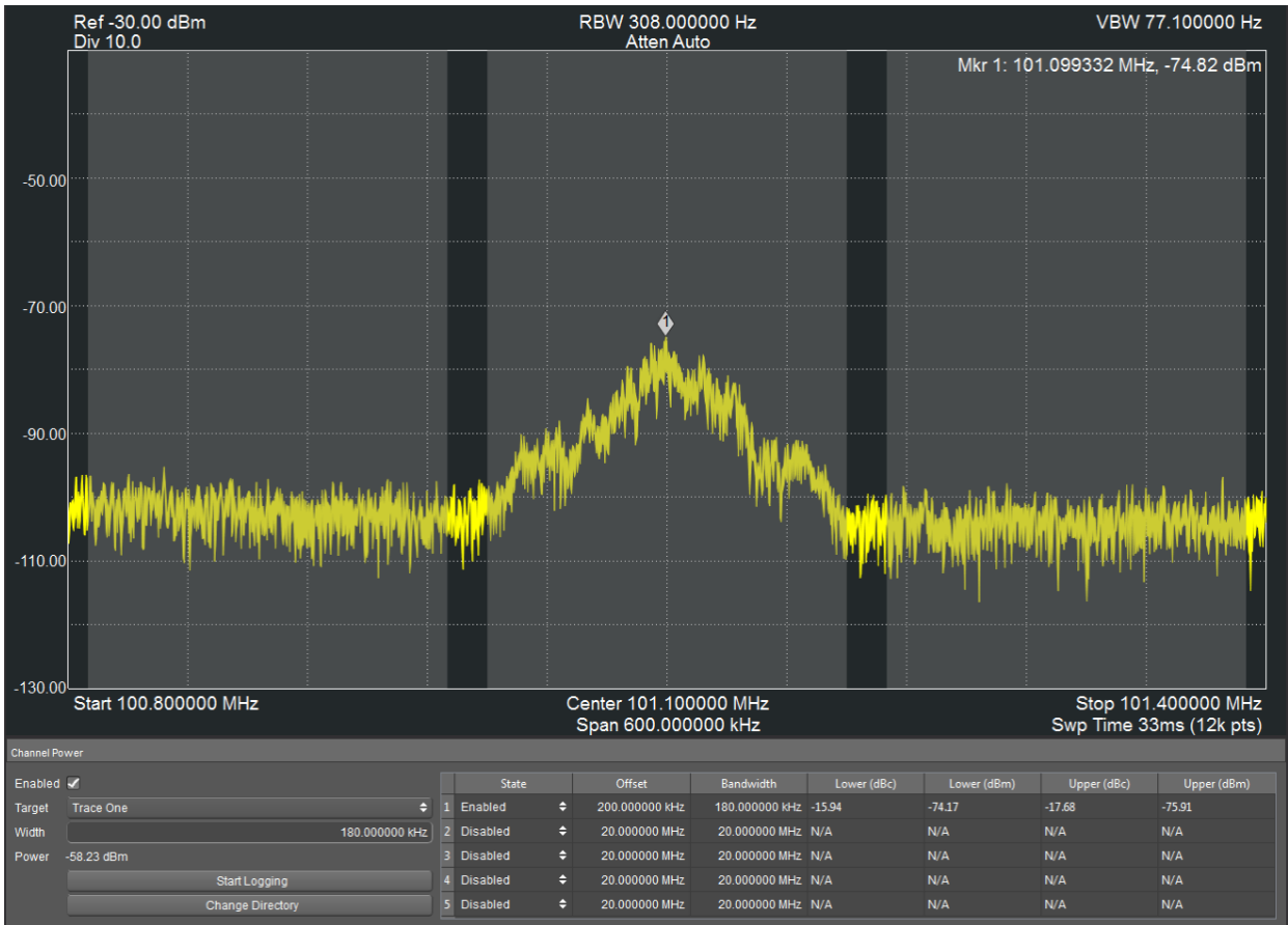
Figure 64: Channel Power on a Broadcast FM Signal
