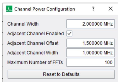
Figure 13: Configuration dialog for the Zero Span Channel Power plot.
