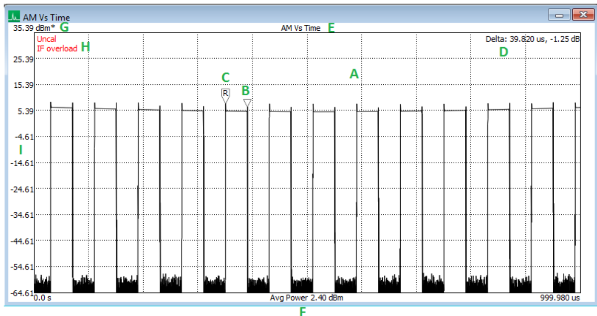
Figure 83: Basic plot areas of interest.
