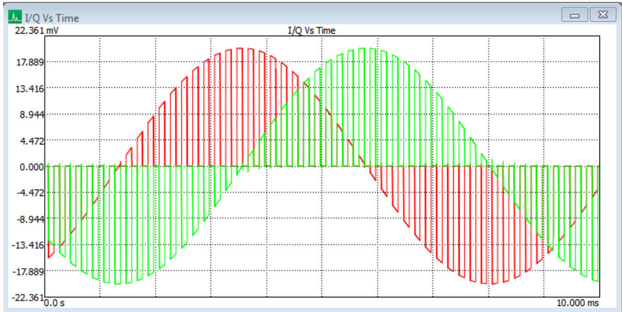
Figure 8: Pulsed CW
