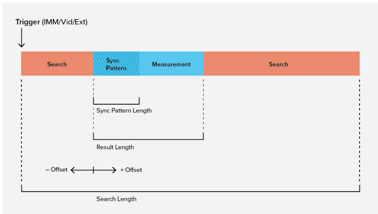
Figure 19: This diagram illustrates how sync search is performed and how the measurement is framed within the search length.
