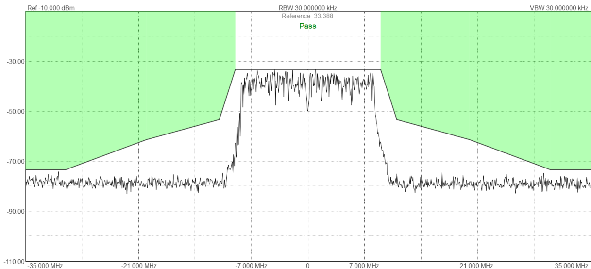
Figure 46: Testing input against an 802.11 OFDM transmission mask.
