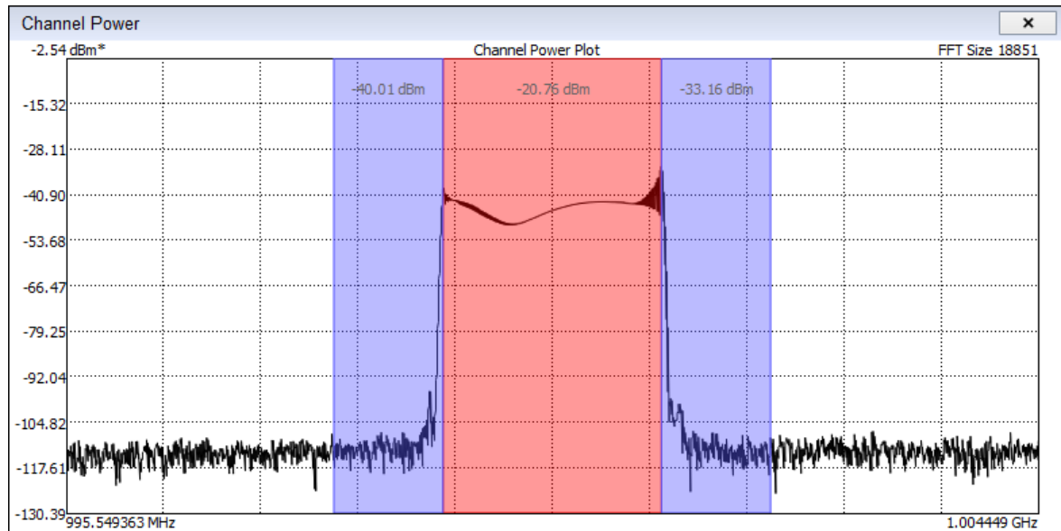
Figure 12: Measuring main and adjacent channels of an FM signal in Zero Span's Channel Power plot.
