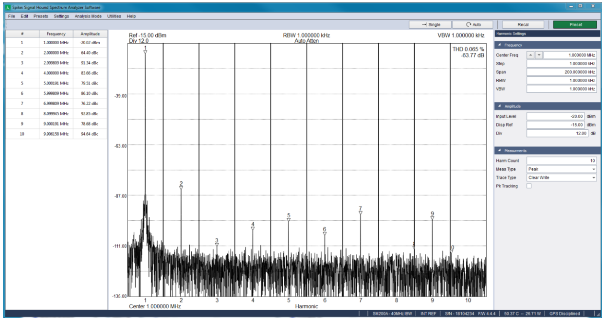
Figure 15: Carrier frequency at 1MHz and 9 harmonics.
