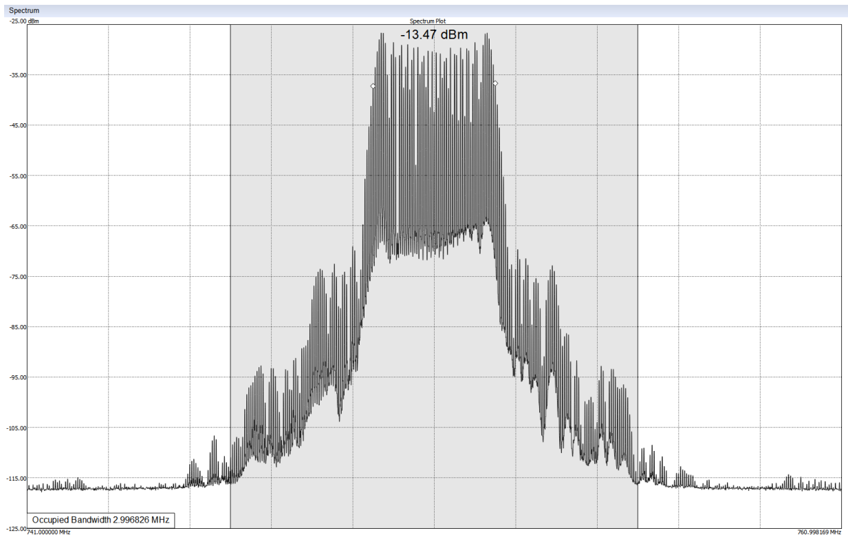
Figure 56: Channel power spectrum plot showing an FM signal.
