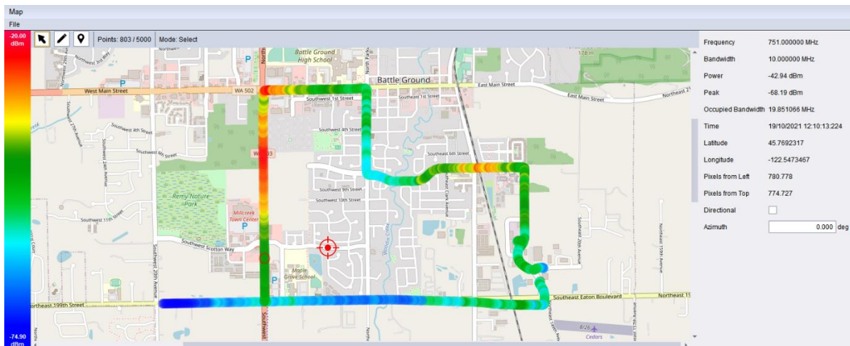
Figure 55: Map view with heat mapped measurements taken of a cell tower signal.
