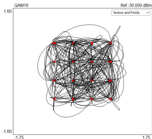
Figure 22: Constellation Diagram for a QAM 16 Input Signal
