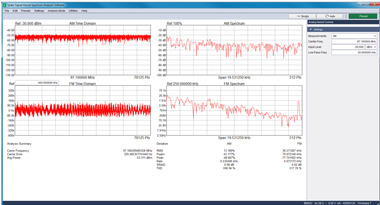
Figure 32: Viewing a broadcast FM signal and observing the 19kHz FM pilot tone in analog demodulation mode.
