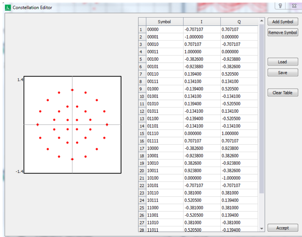
Figure 18: APSK32 in the constellation editor.
