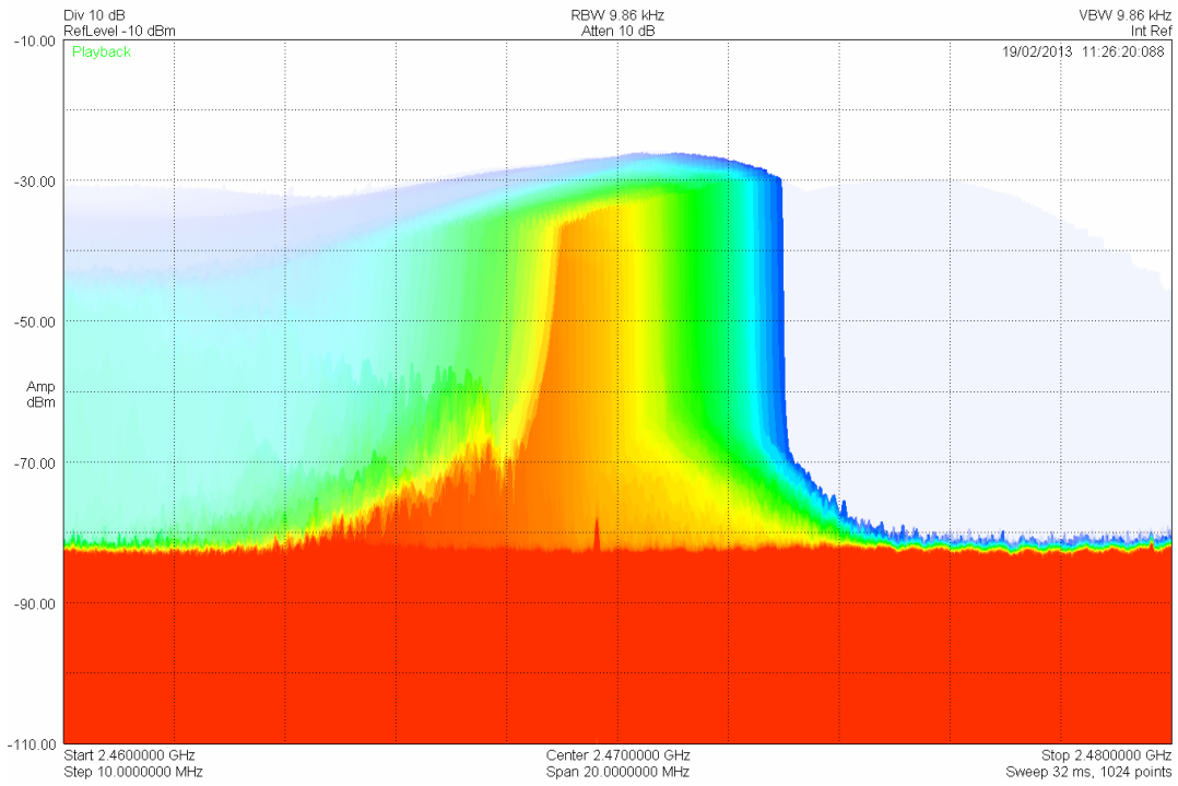
Figure 87: Sweep mode persistence showing the signal from a poorly shielded commercial microwave oven.
