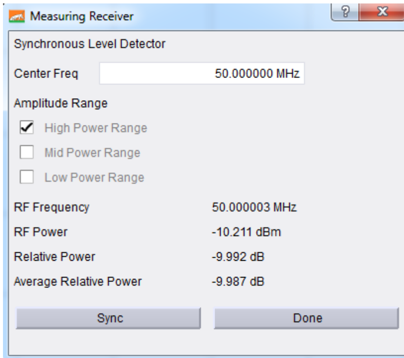
Figure 67: Measuring Receiver Control Dialog
