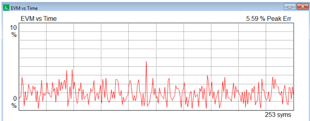
Figure 24: EVM vs Time plot
