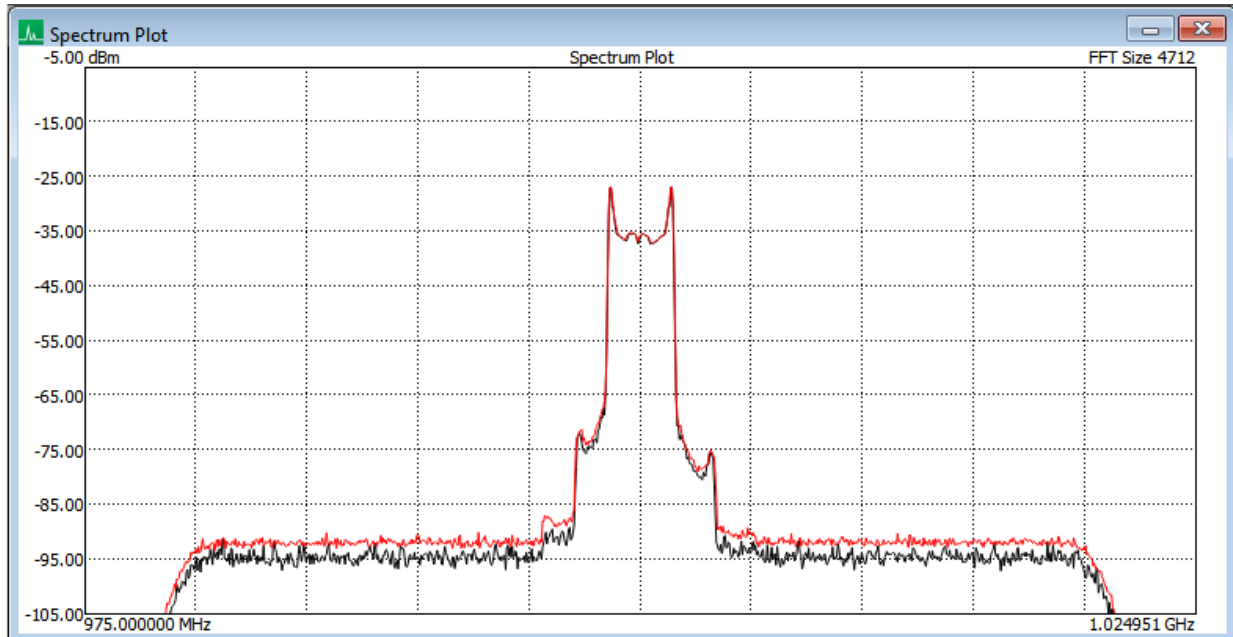
Figure 9: FM signal with max hold.
