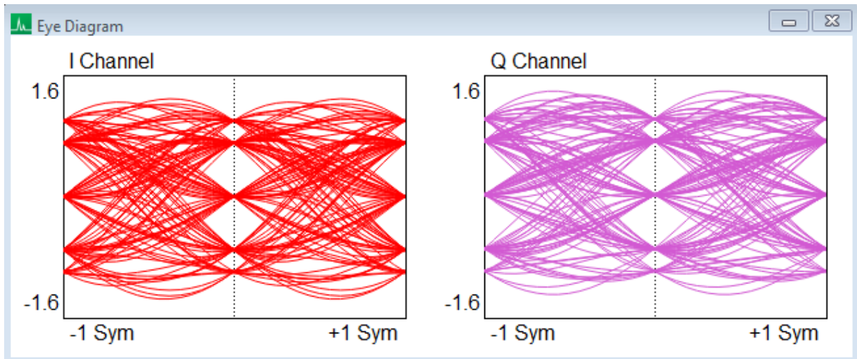
Figure 23: Eye diagram for a Pi/4DQPSK signal
