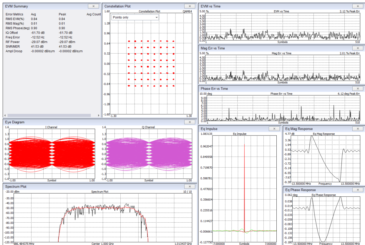
Figure 20: Characterizing a QAM64 waveform over a heavily impaired channel using equalization.
