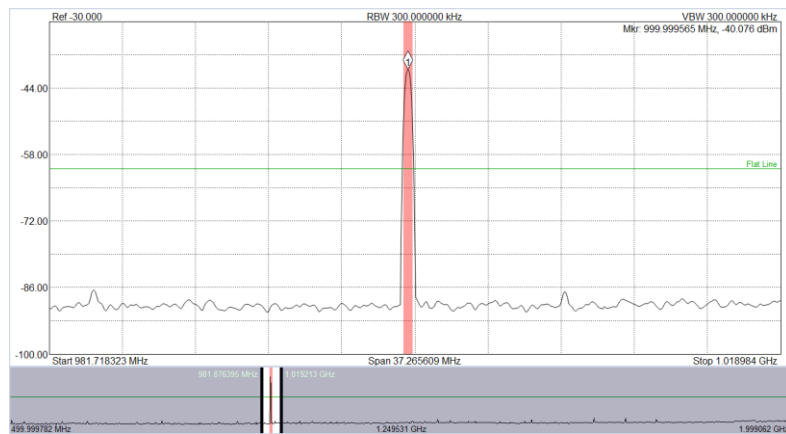
Figure 39: Regional zoom being used for close inspection of event.
