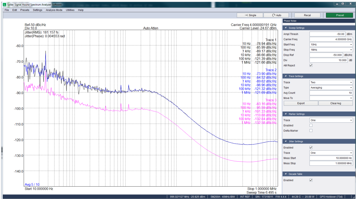
Figure 17: SM200A measuring the phase noise of a signal generator at 1 and 4 GHz carriers.
