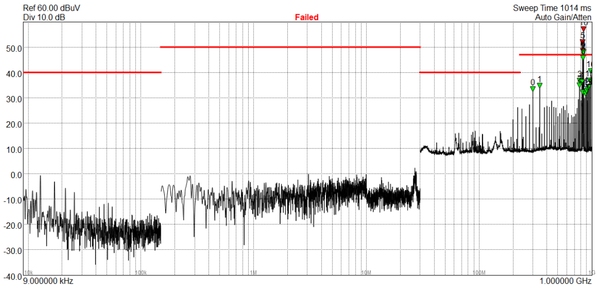
Figure 27: Frequency Scan Display Showing Four Configured Sweep Ranges.
