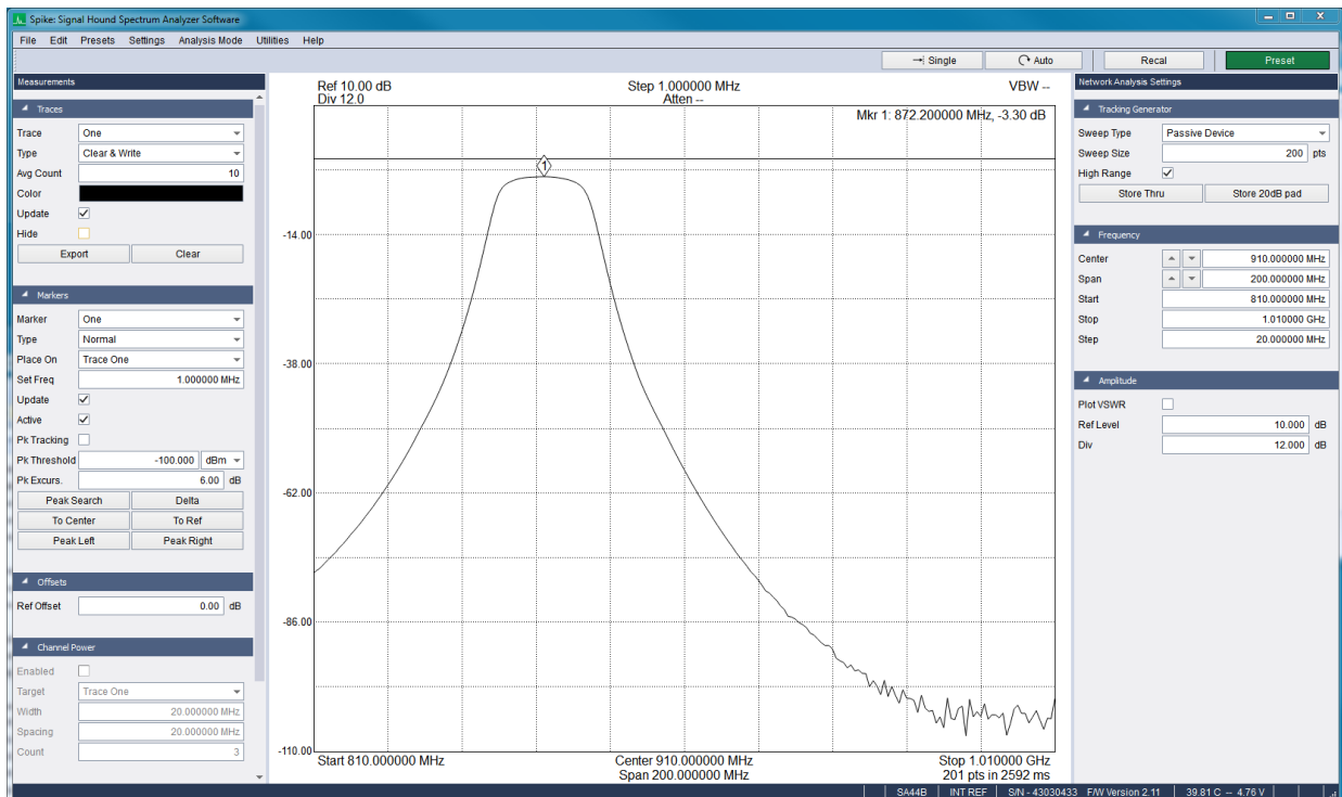
Figure 16 The SA44B and TG44A sweeping a passive bandpass filter.
